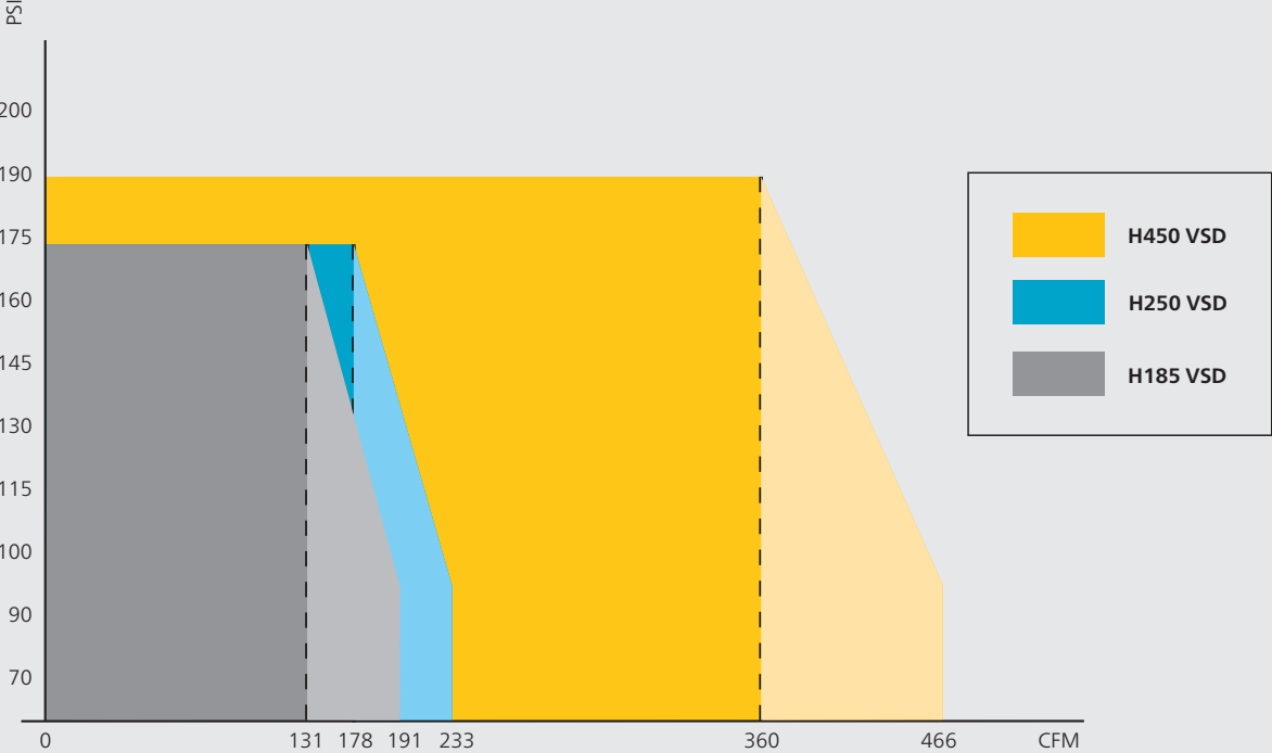
Operating range E-Air VSD
